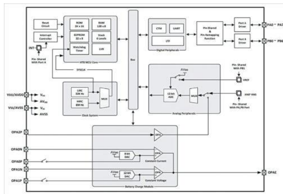
Figure.2. EV Charger Circuit Diagram
